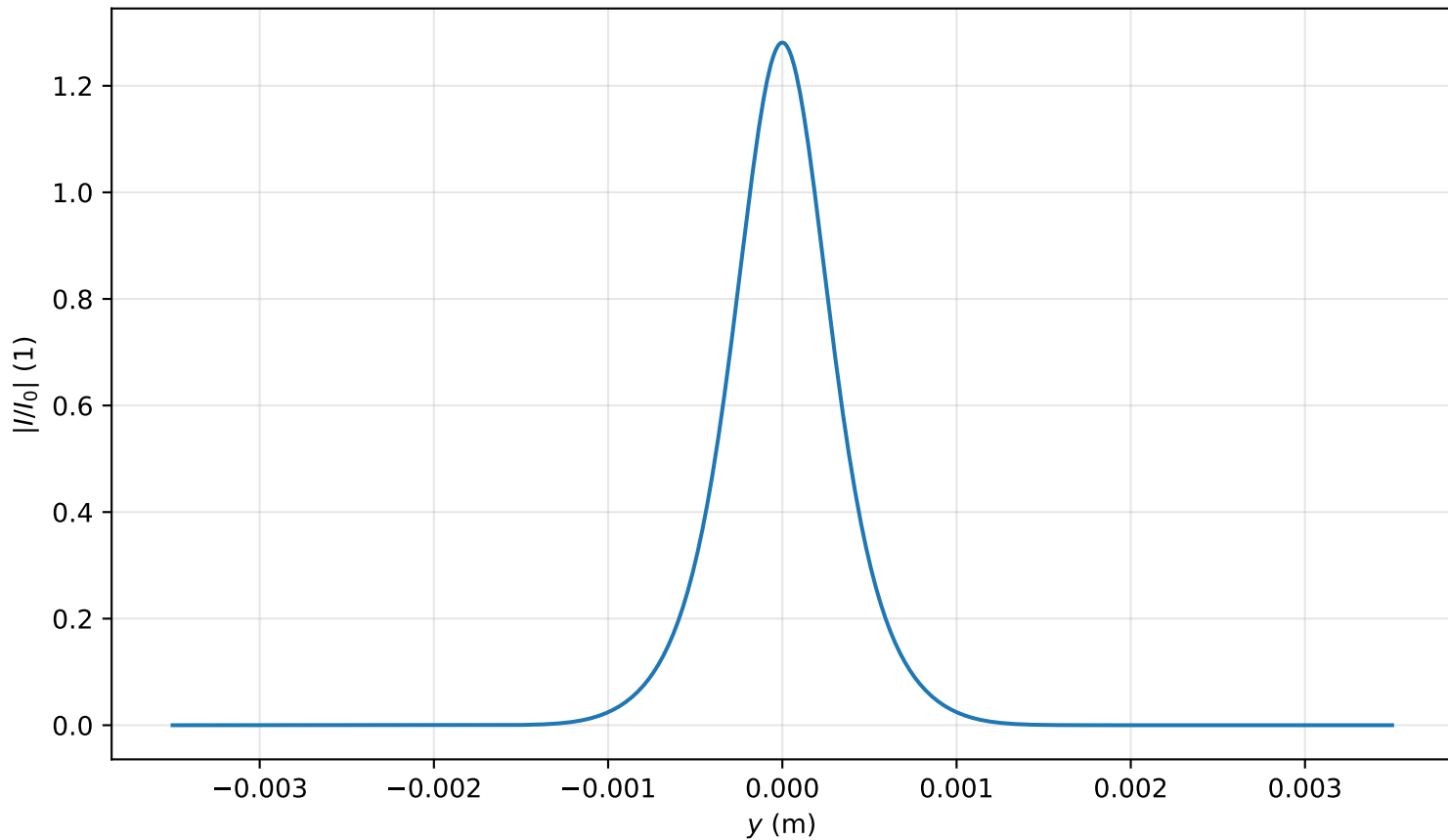
Intensity profile I(x=0, y, z=0.955)/I_0 , P_{in}=0.8P_{cr} , artificial time
